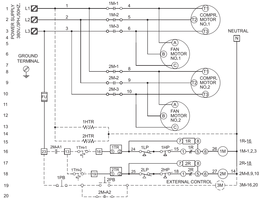
CONNECTION DIAGRAM
