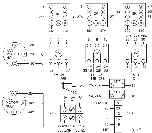
CONNECTION DIAGRAM
