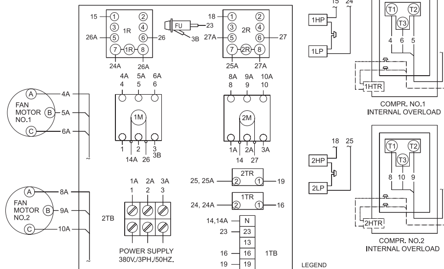
CONNECTION DIAGRAM
